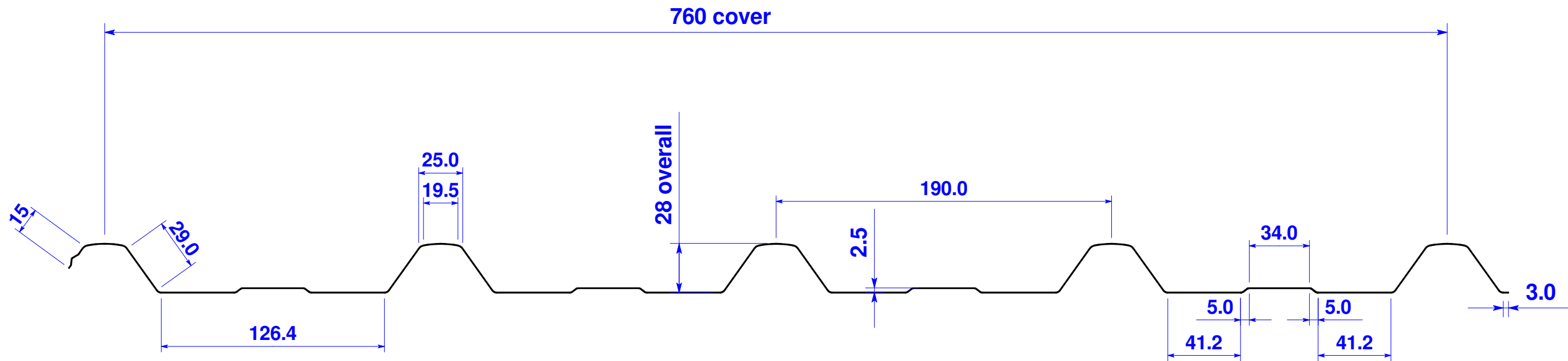
5-Rib - 760mm cover 940mm coil feed 0.40G550 / 0.55G300 & G550
