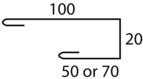
Window Side & Sill Flashings
