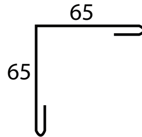
External Corner Over Flashing
