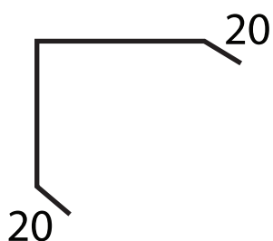
External Corner Vertical Cladding
