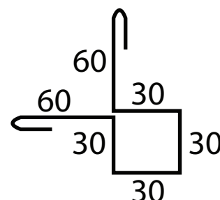
Boc Corner Flashing
