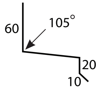
Window & Door Head Flashing
