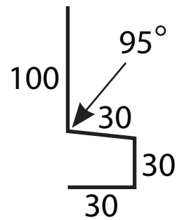
Base Flashing
